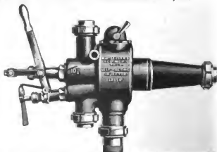
Fig. 3107. Sellers' Class P, Self-Acting Injector for Back Head of Boiler.
